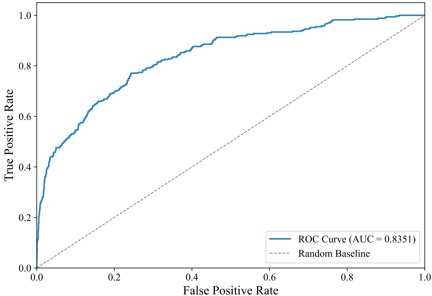
ROC Curve — GERMAN_MANUAL (intfloat/multilingual-e5-large-instruct, Random_Forest_Optimized)
