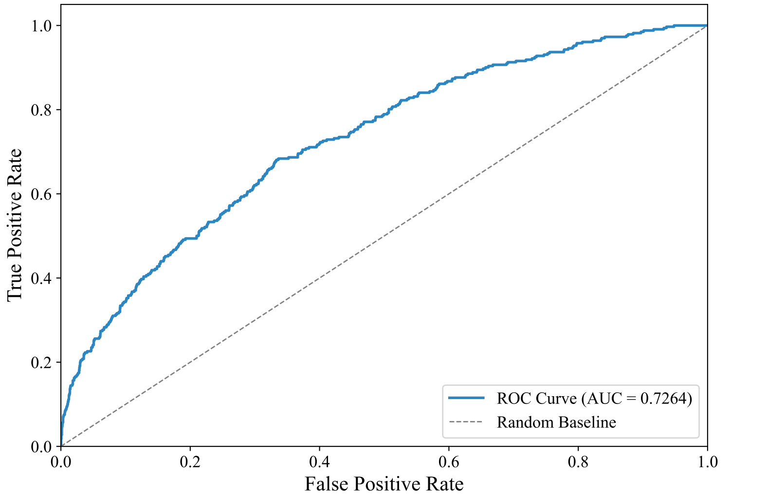
ROC Curve — GERMAN_MANUAL (paraphrase-multilingual-MiniLM-L12-v2, Random_Forest_Optimized)
