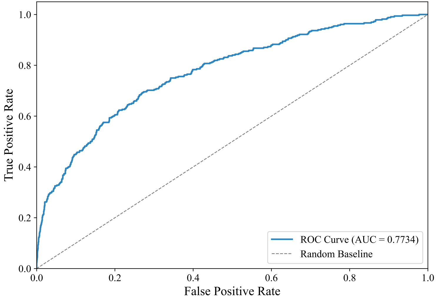
ROC Curve — GERMAN_MANUAL (paraphrase-multilingual-MiniLM-L12-v2, XGBoost)
