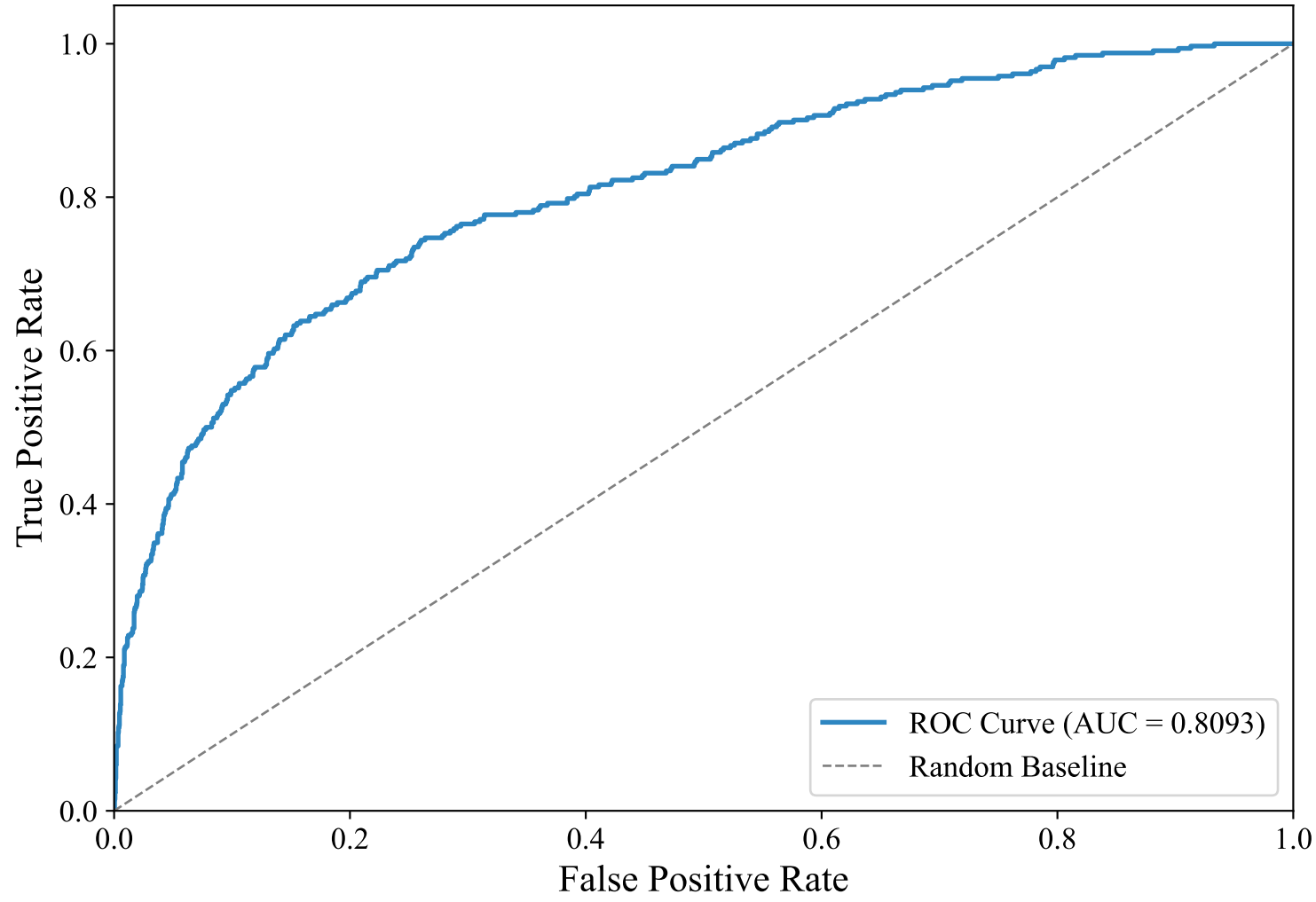
ROC Curve — GERMAN_MANUAL (paraphrase-multilingual-mpnet-base-v2, Voting_Ensemble)
