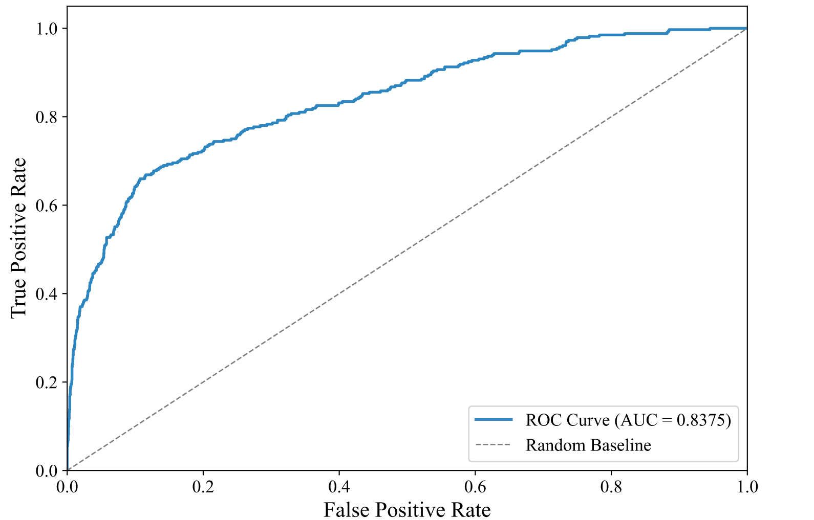
ROC Curve — GERMAN_MANUAL (snowflake-arctic-embed-l-v2.0, LightGBM)
