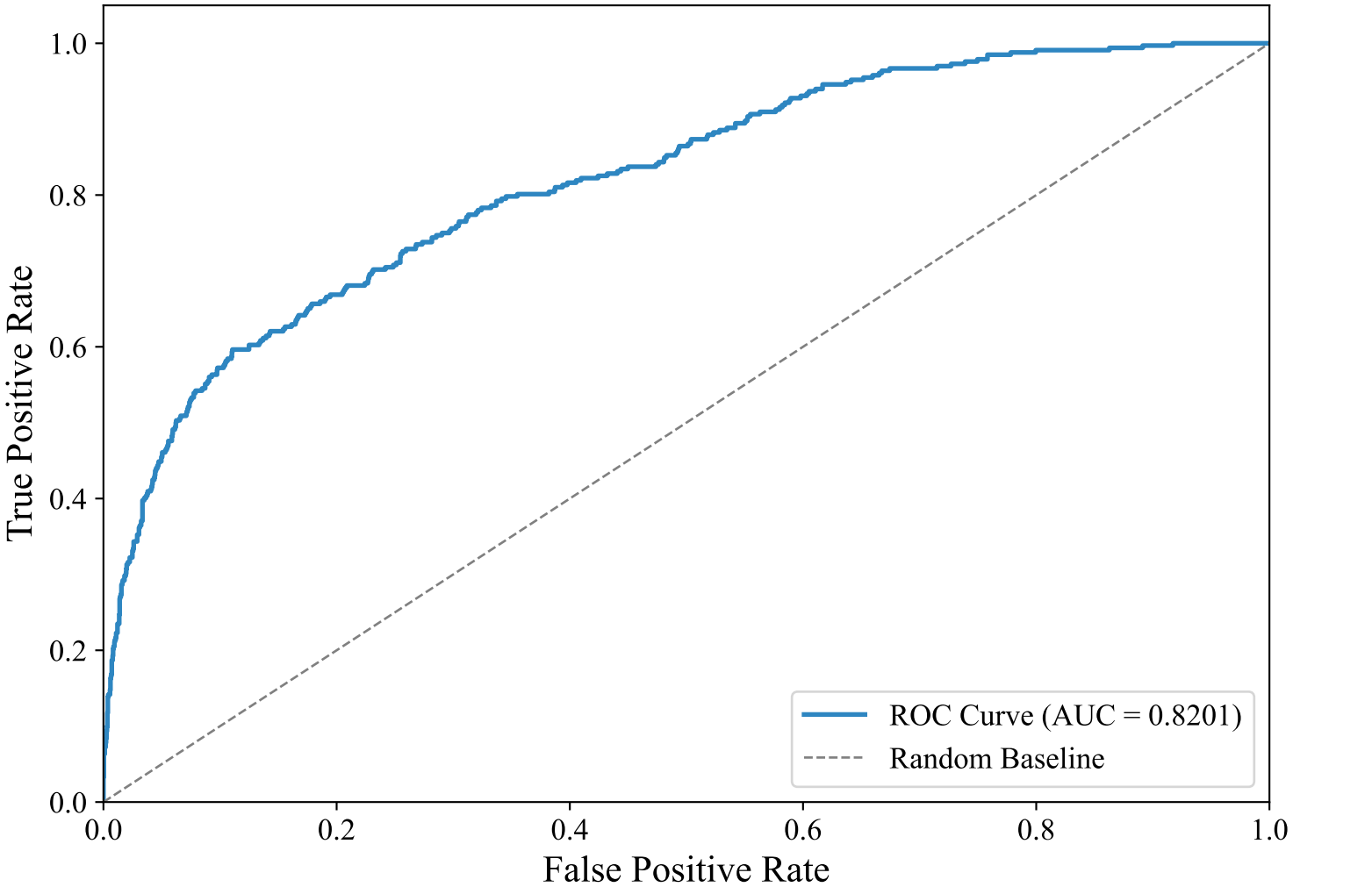
ROC Curve — GERMAN_MANUAL (xlm-roberta-base, Voting_Ensemble)
