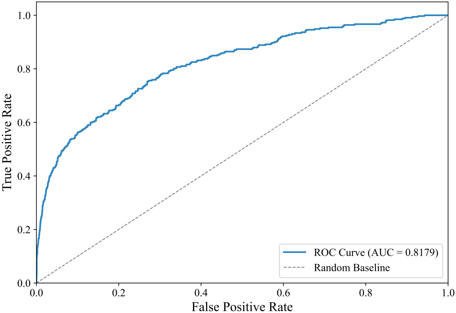
ROC Curve — GERMAN_MANUAL (xlm-roberta-base, XGBoost_Optimized)
