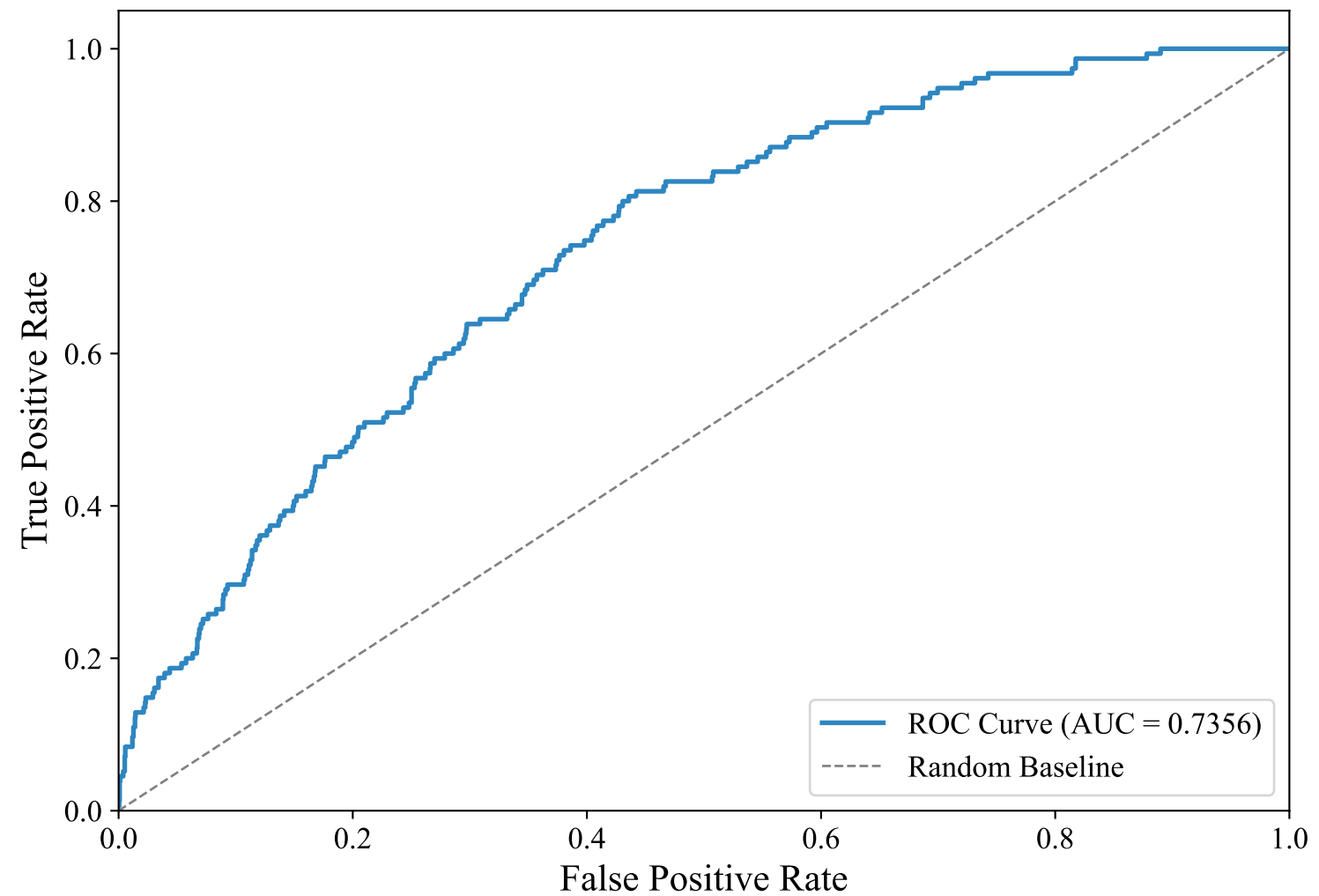
ROC Curve — SWEDISH_MANUAL (bert-base-multilingual-uncased, LightGBM_Optimized)
