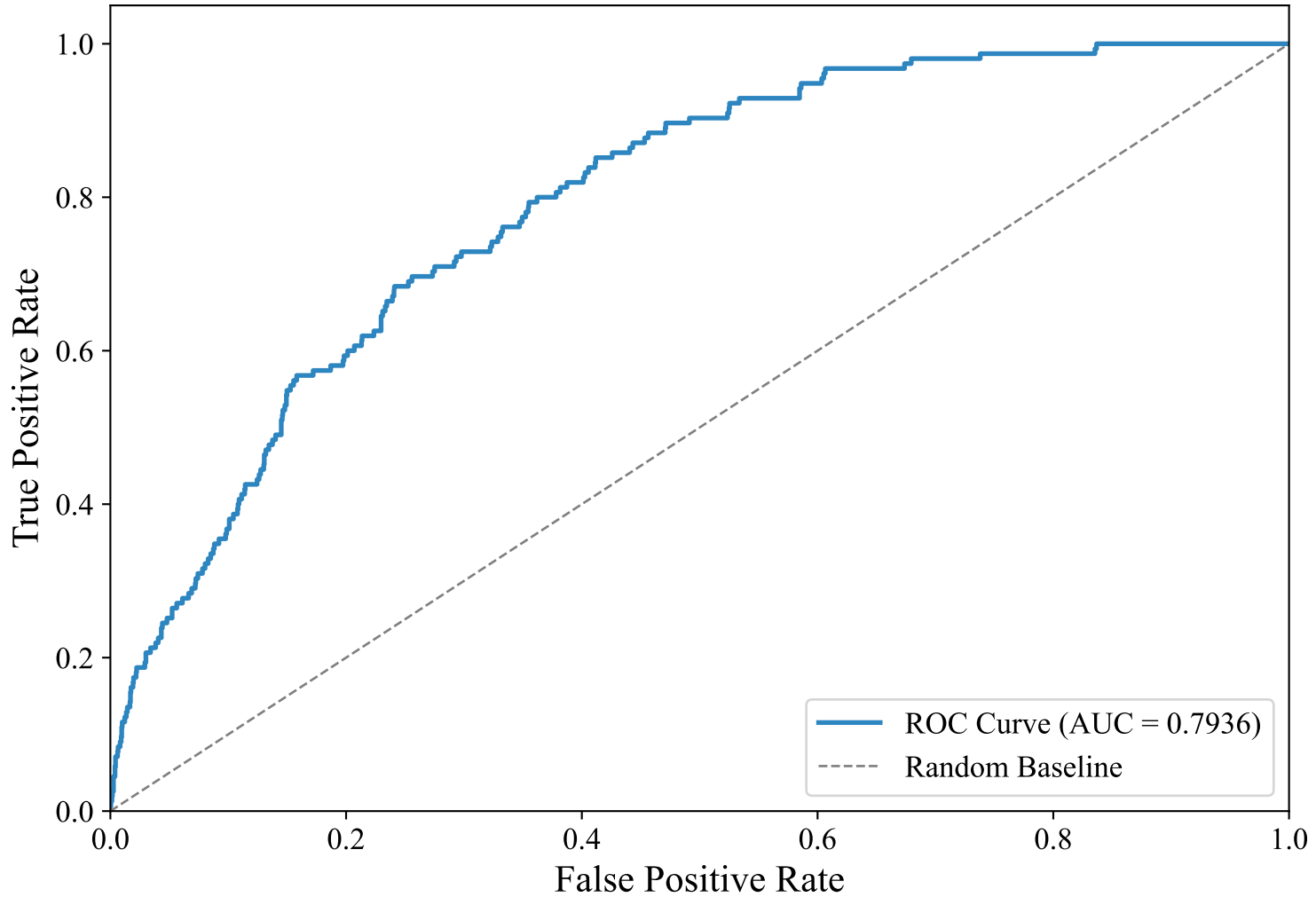
ROC Curve — SWEDISH_MANUAL (efederici/e5-base-multilingual-4096, LightGBM_Optimized)
