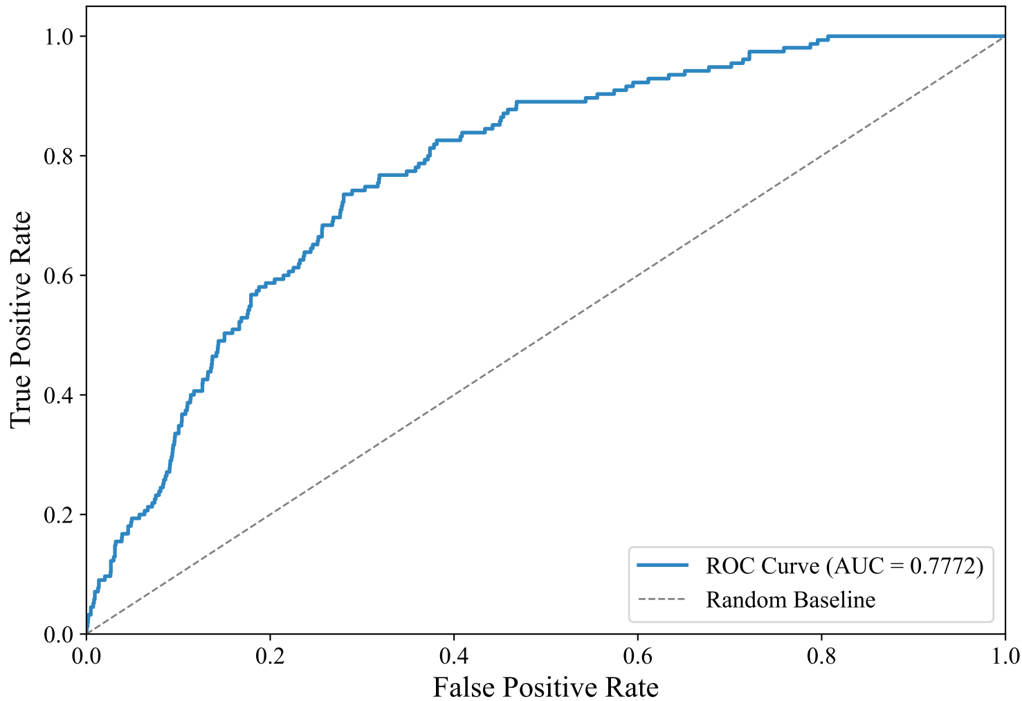
ROC Curve — SWEDISH_MANUAL (efederici/e5-base-multilingual-4096, Random_Forest_Optimized)
