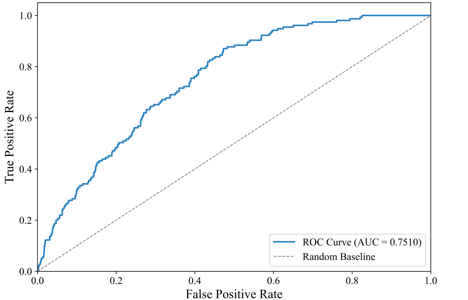
ROC Curve — SWEDISH_MANUAL (paraphrase-multilingual-MiniLM-L12-v2, Random_Forest_Optimized)
