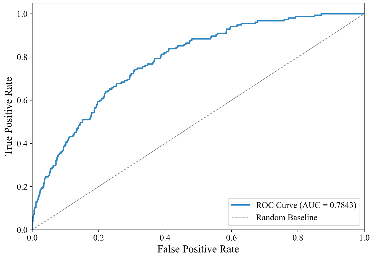
ROC Curve — SWEDISH_MANUAL (paraphrase-multilingual-mpnet-base-v2, LightGBM)
