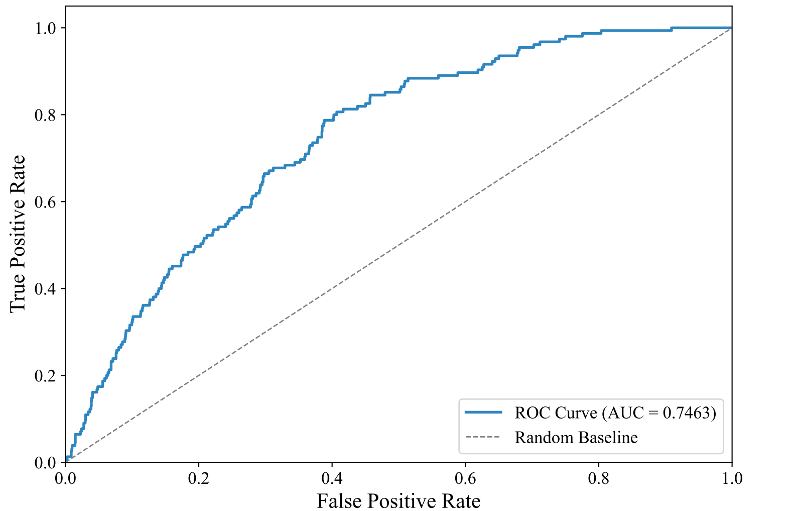
ROC Curve — SWEDISH_MANUAL (paraphrase-multilingual-mpnet-base-v2, Random_Forest)
