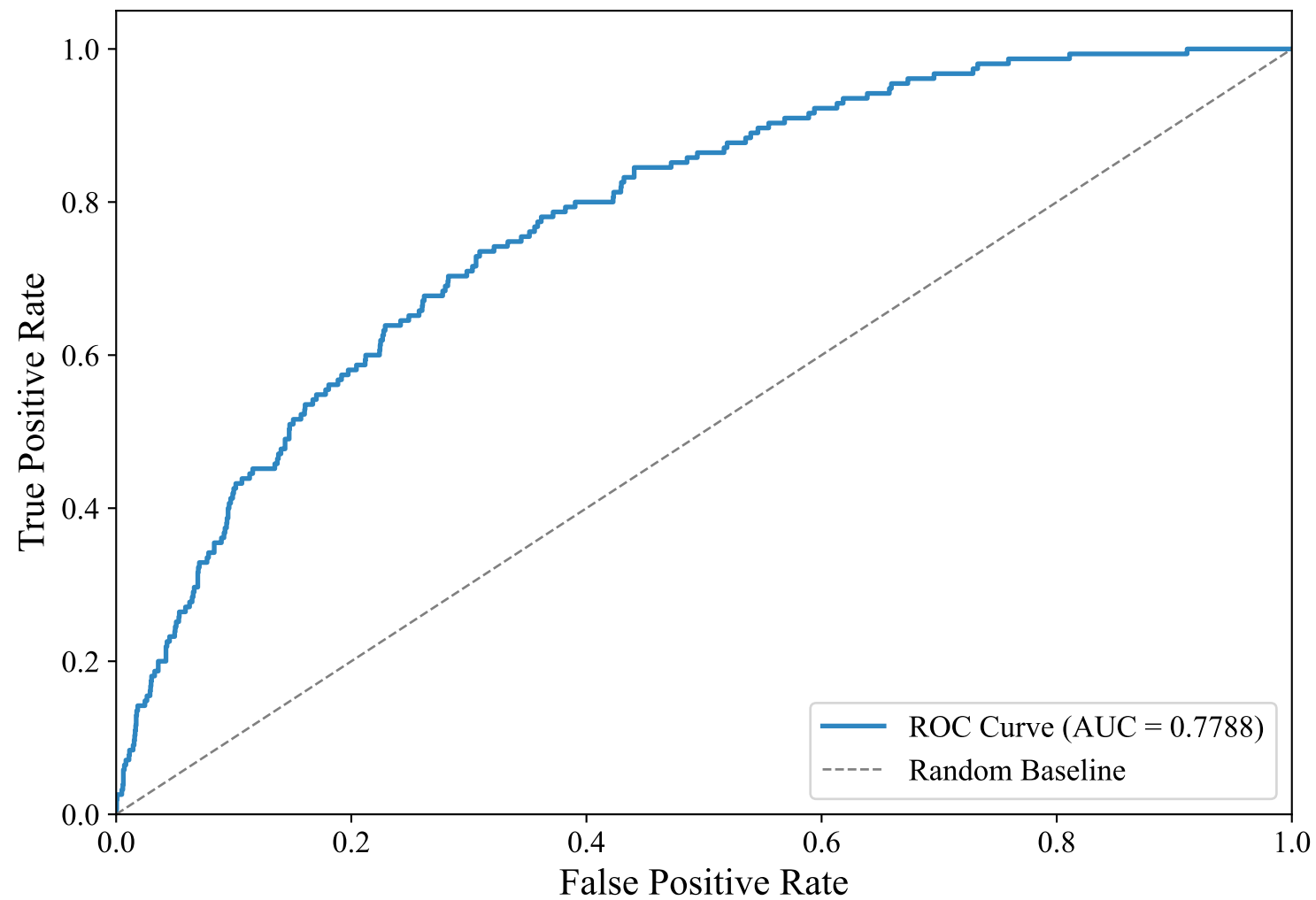
ROC Curve — SWEDISH_MANUAL (paraphrase-multilingual-mpnet-base-v2, Voting_Ensemble)
