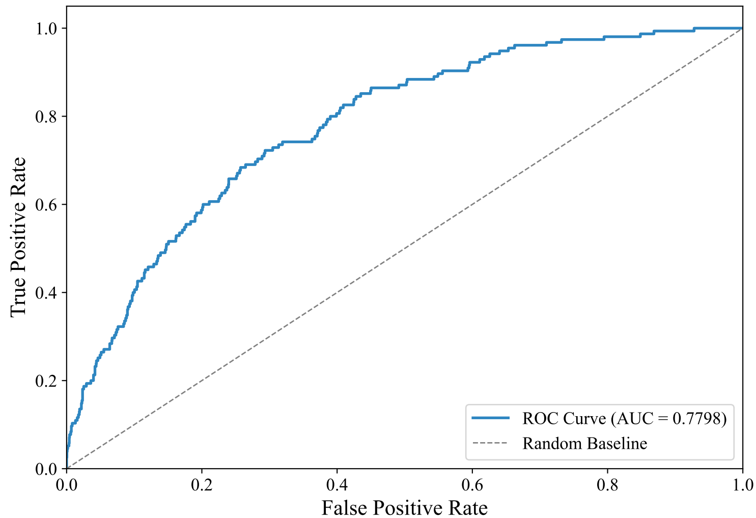
ROC Curve — SWEDISH_MANUAL (paraphrase-multilingual-mpnet-base-v2, XGBoost)
