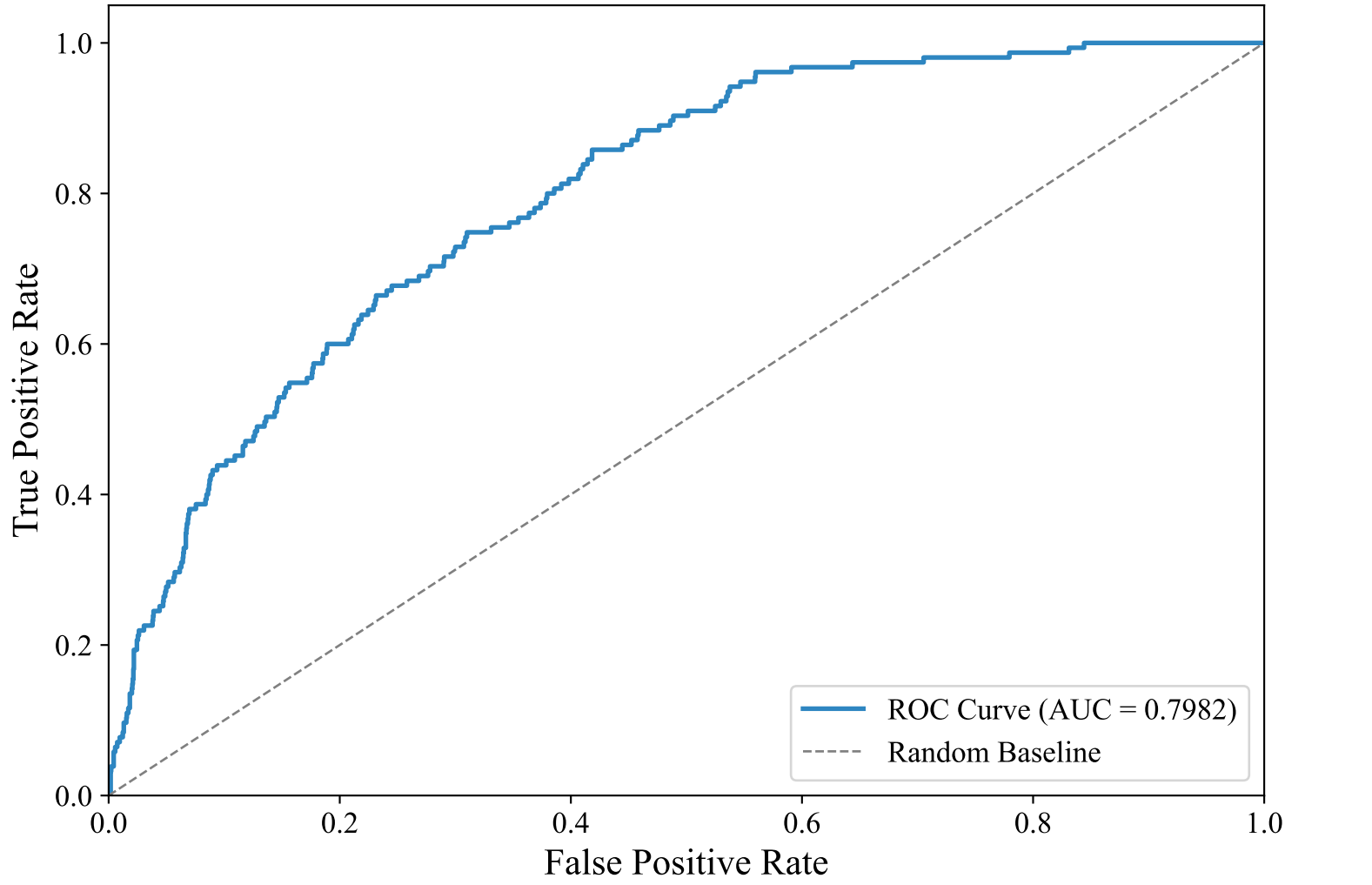
ROC Curve — SWEDISH_MANUAL (snowflake-arctic-embed-l-v2.0, LightGBM)
