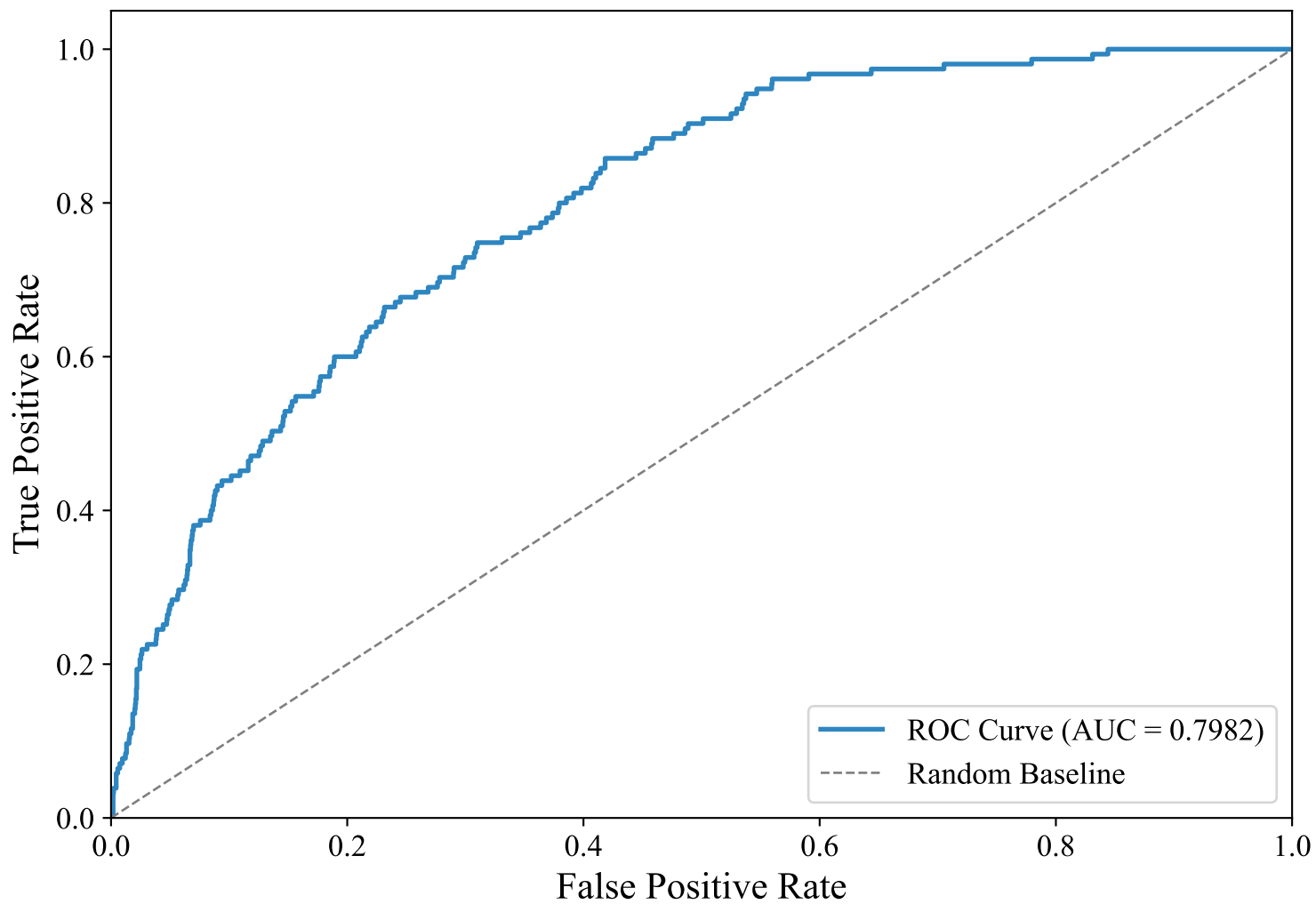
ROC Curve — SWEDISH_MANUAL (snowflake-arctic-embed-l-v2.0, LightGBM_Optimized)
