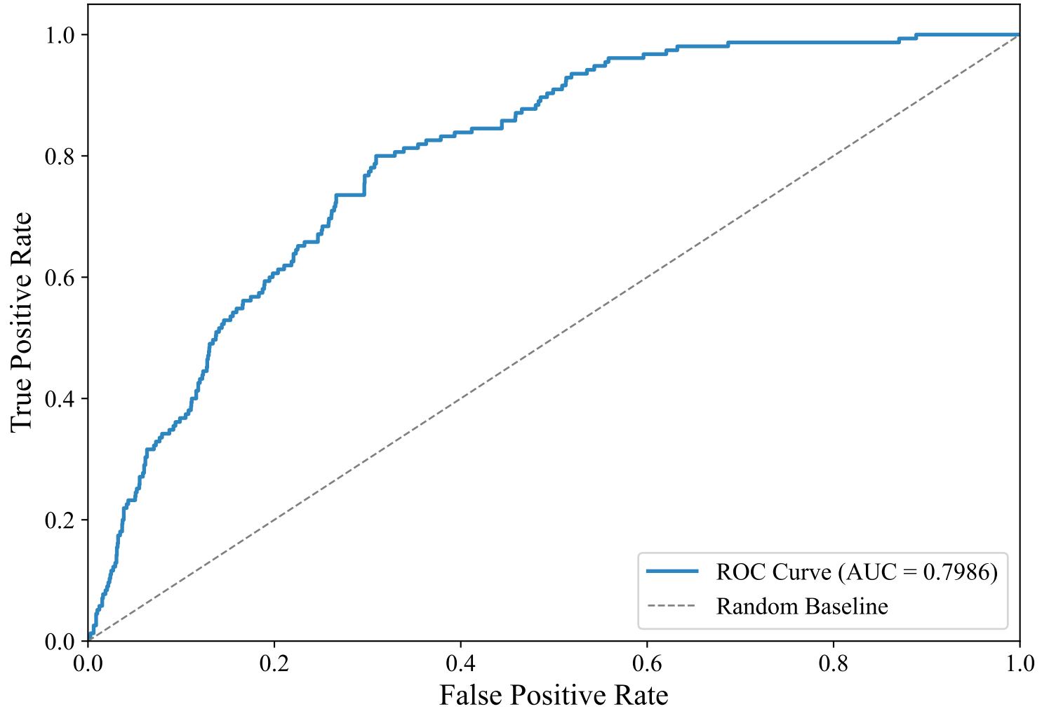
ROC Curve — SWEDISH_MANUAL (snowflake-arctic-embed-l-v2.0, Random_Forest_Optimized)
