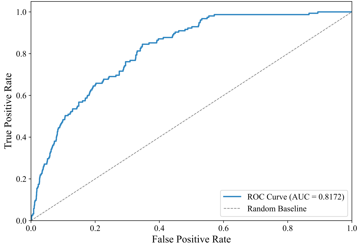
ROC Curve — SWEDISH_MANUAL (snowflake-arctic-embed-l-v2.0, Voting_Ensemble)
