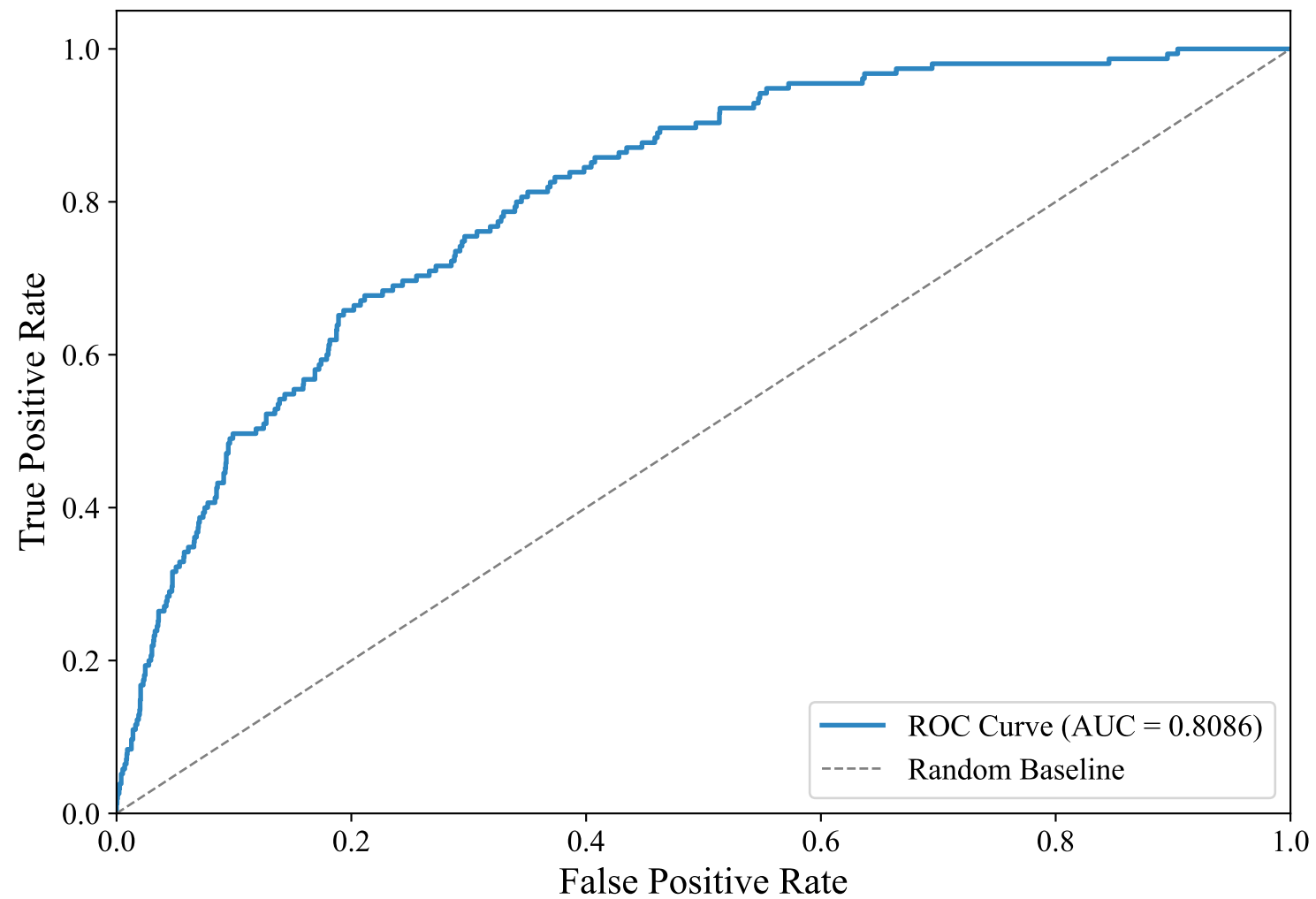
ROC Curve — SWEDISH_MANUAL (snowflake-arctic-embed-l-v2.0, XGBoost)
