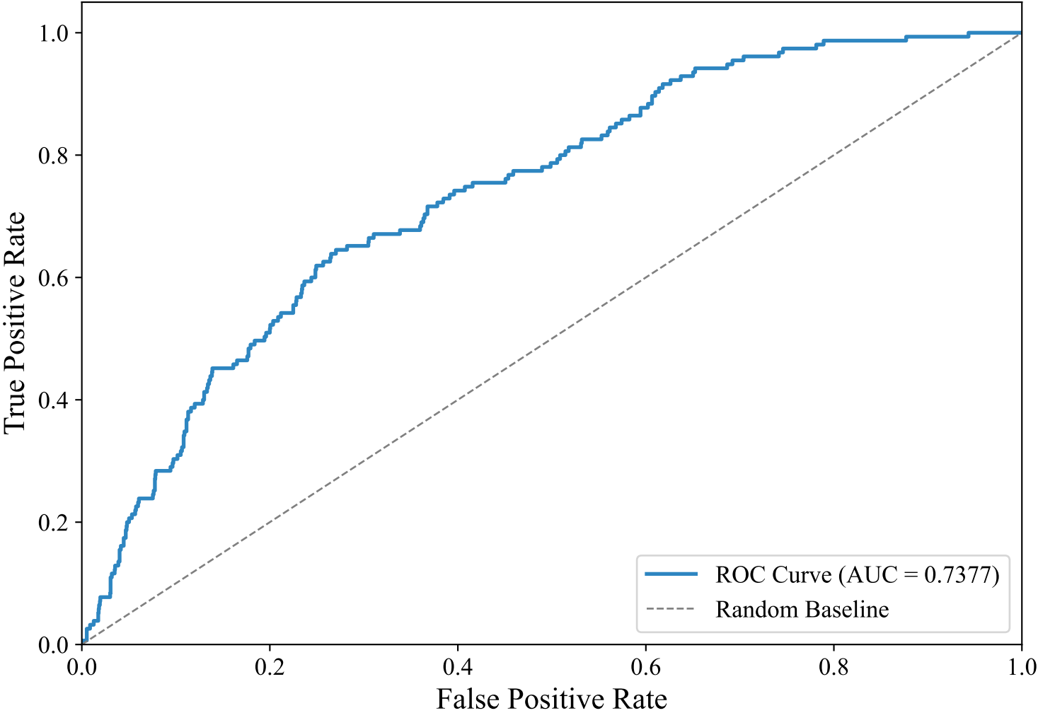
ROC Curve — SWEDISH_MANUAL (xlm-roberta-base, Random_Forest)
