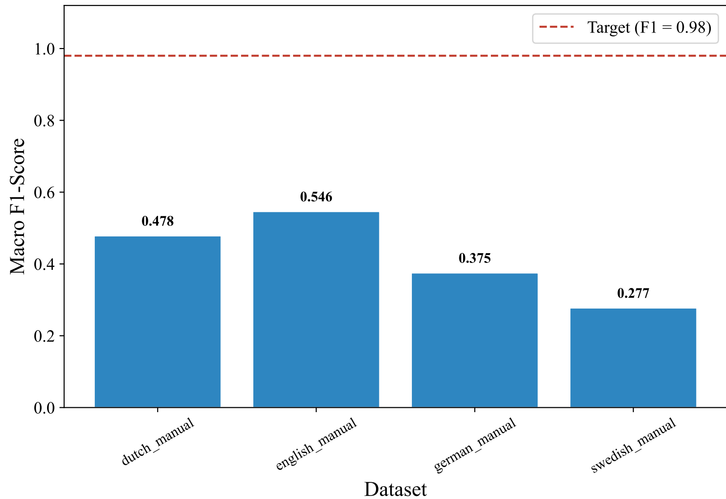
Best Macro-F1 by Dataset — Iteration 6
