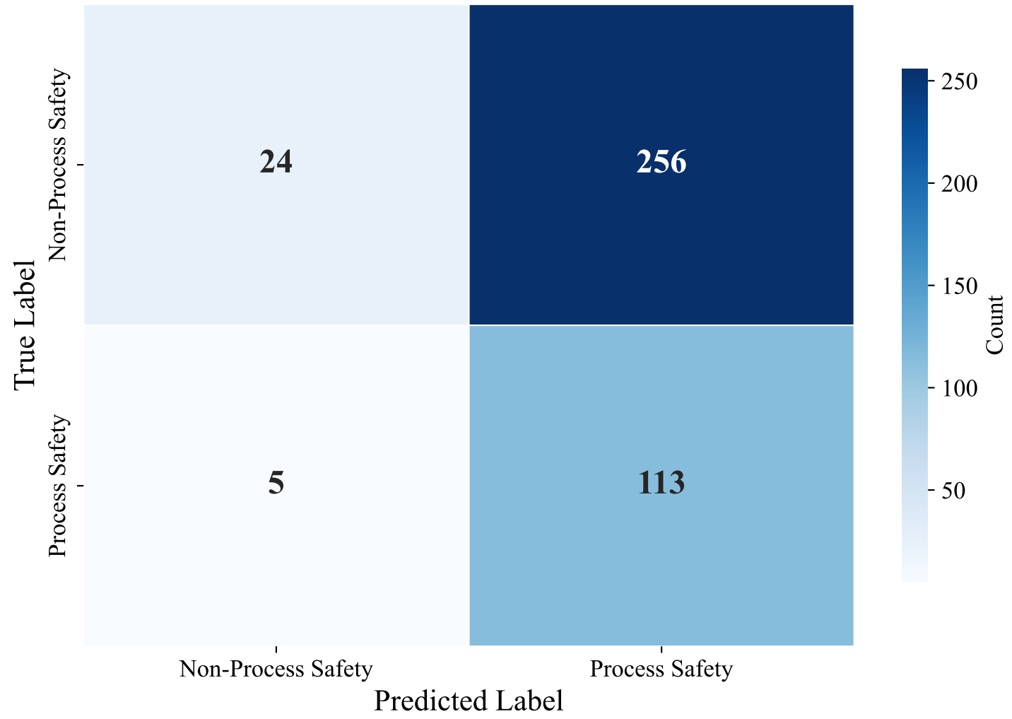
Confusion Matrix — DUTCH_MANUAL (bert-base-multilingual-uncased, svm_rbf)
