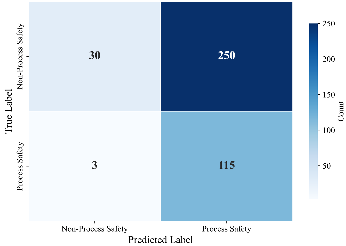
Confusion Matrix — DUTCH_MANUAL (multilingual-e5-large-instruct, xgboost)
