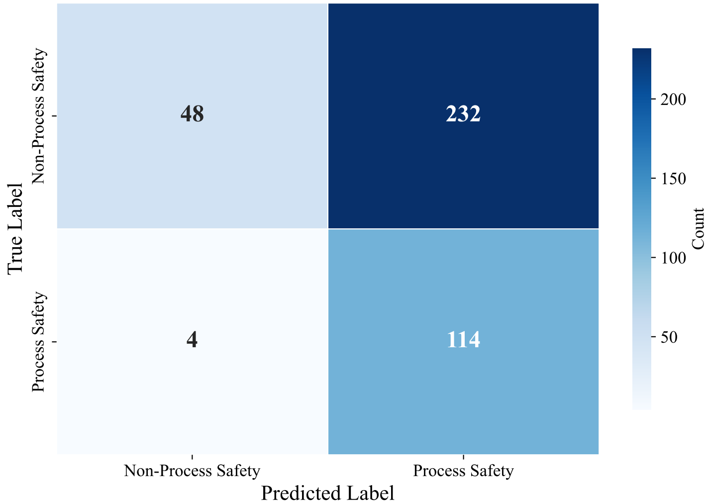
Confusion Matrix — DUTCH_MANUAL (paraphrase-multilingual-MiniLM-L12-v2, lightgbm)
