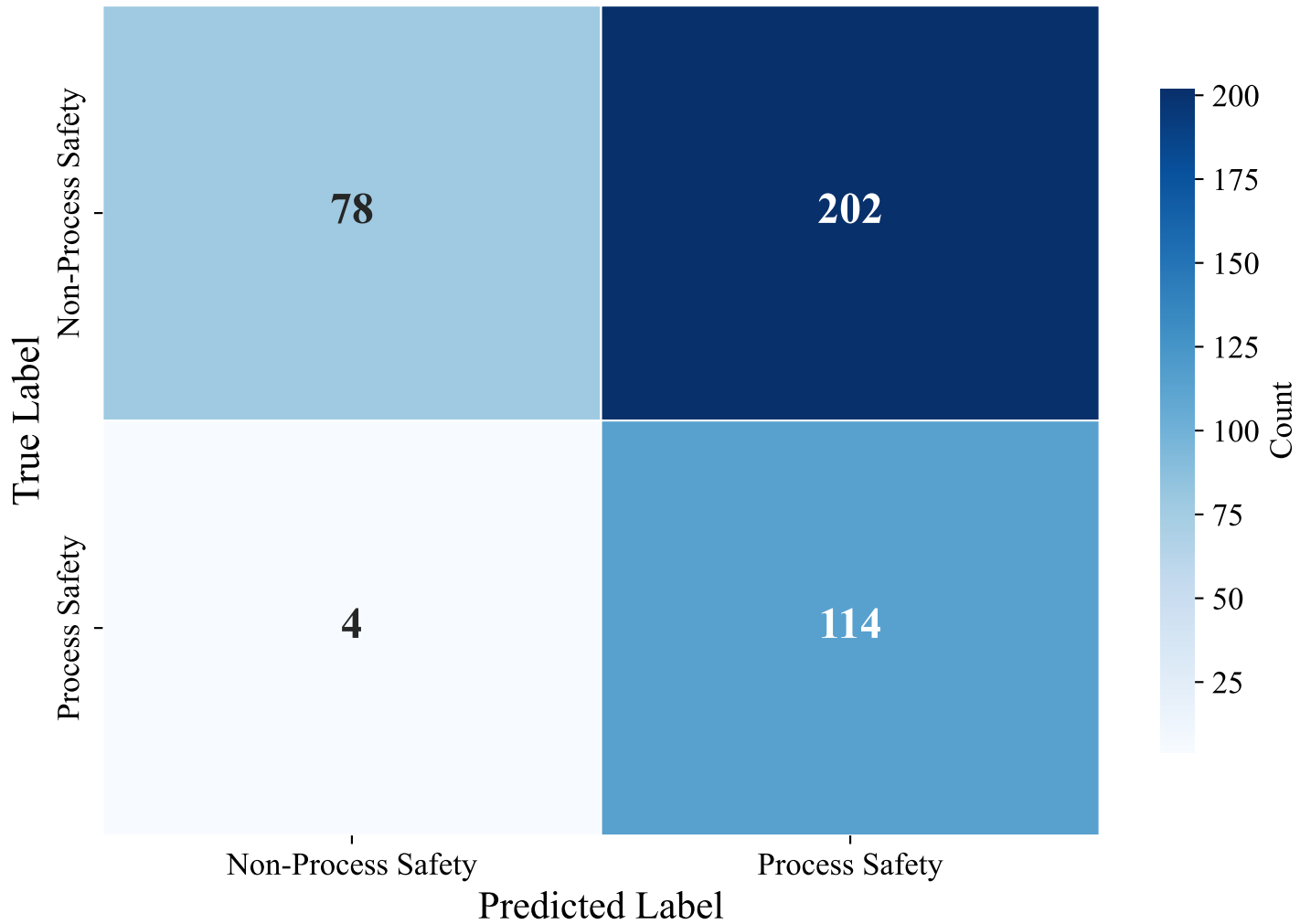
Confusion Matrix — DUTCH_MANUAL (paraphrase-multilingual-mpnet-base-v2, lightgbm)
