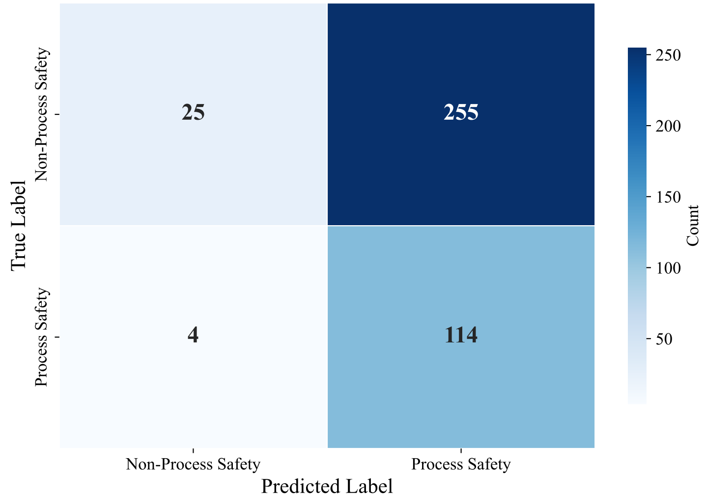
Confusion Matrix — DUTCH_MANUAL (paraphrase-multilingual-mpnet-base-v2, random_forest)
