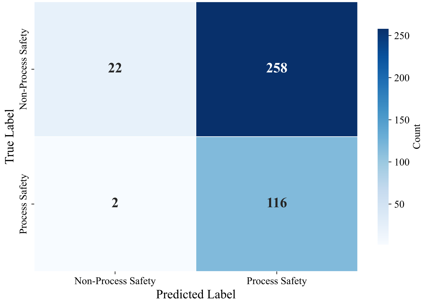
Confusion Matrix — DUTCH_MANUAL (snowflake-arctic-embed-l-v2.0, lightgbm)
