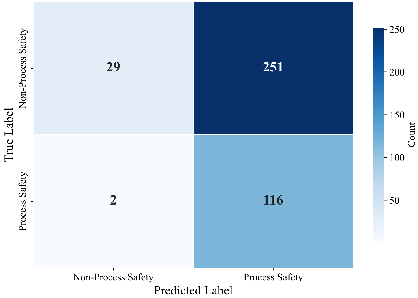
Confusion Matrix — DUTCH_MANUAL (snowflake-arctic-embed-l-v2.0, svm_linear)
