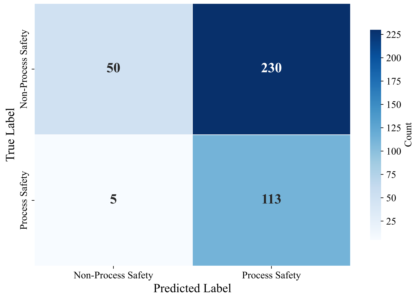
Confusion Matrix — DUTCH_MANUAL (snowflake-arctic-embed-l-v2.0, svm_rbf)
