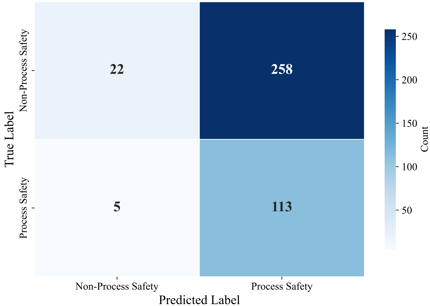
Confusion Matrix — DUTCH_MANUAL (snowflake-arctic-embed-l-v2.0, xgboost)
