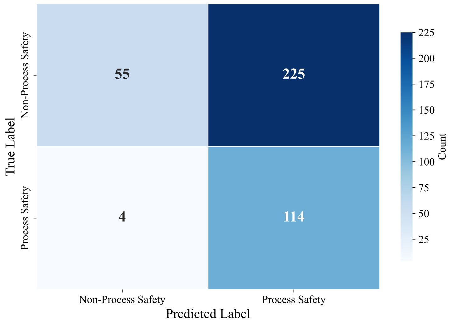
Confusion Matrix — DUTCH_MANUAL (xlm-roberta-base, svm_linear)
