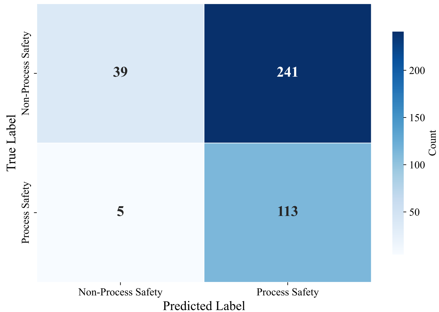
Confusion Matrix — DUTCH_MANUAL (xlm-roberta-base, svm_rbf)
