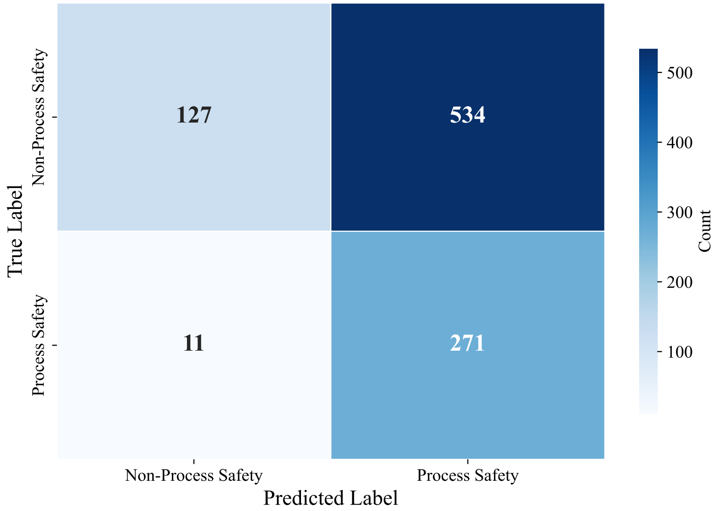
Confusion Matrix — ENGLISH_MANUAL (bert-base-multilingual-uncased, xgboost)
