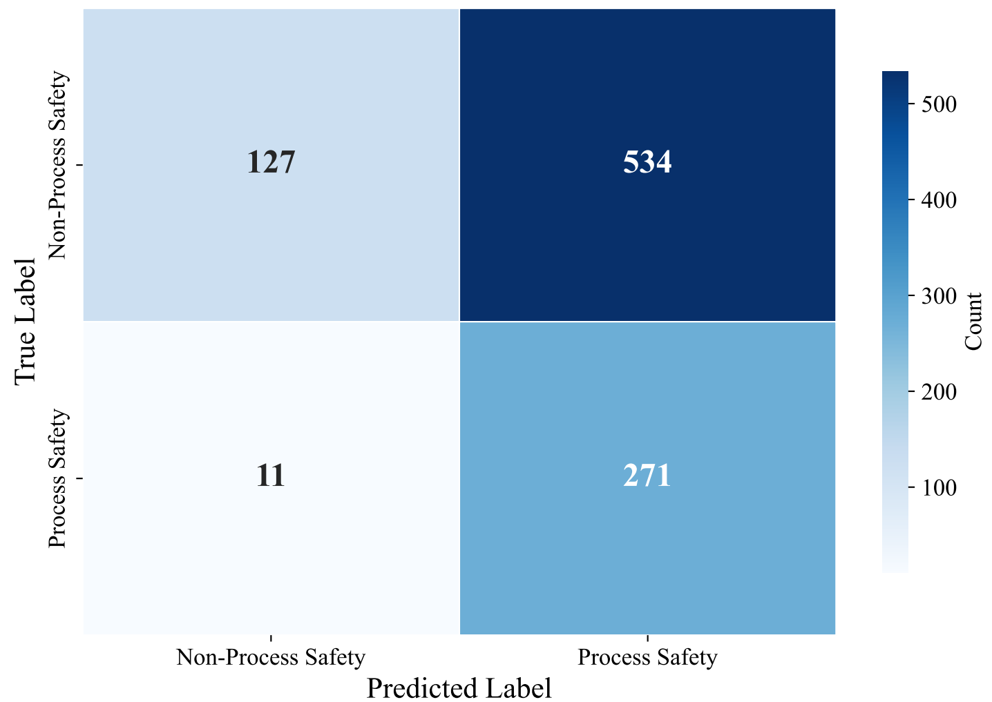
Confusion Matrix — ENGLISH_MANUAL (multilingual-e5-large-instruct, lightgbm)
