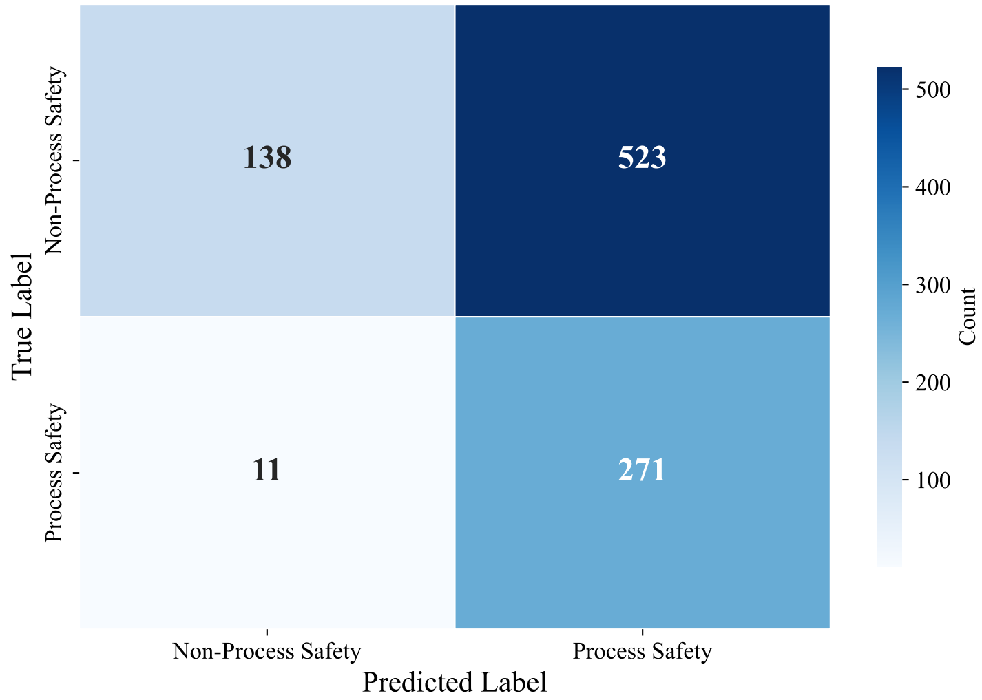
Confusion Matrix — ENGLISH_MANUAL (multilingual-e5-large-instruct, random_forest)
