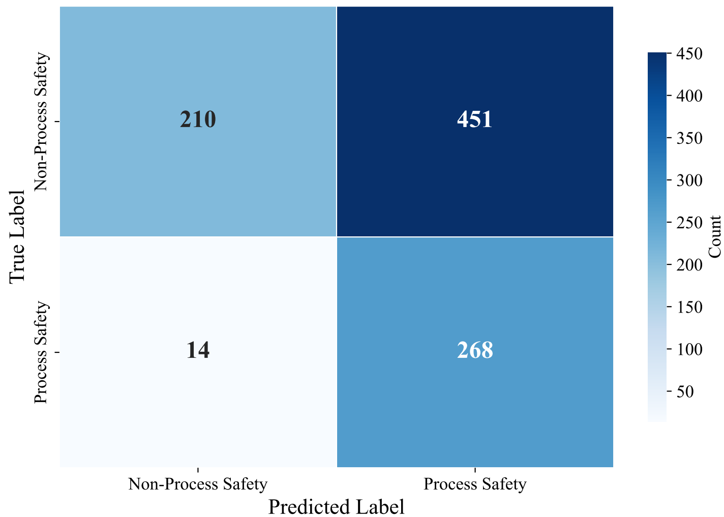
Confusion Matrix — ENGLISH_MANUAL (multilingual-e5-large-instruct, svm_linear)
