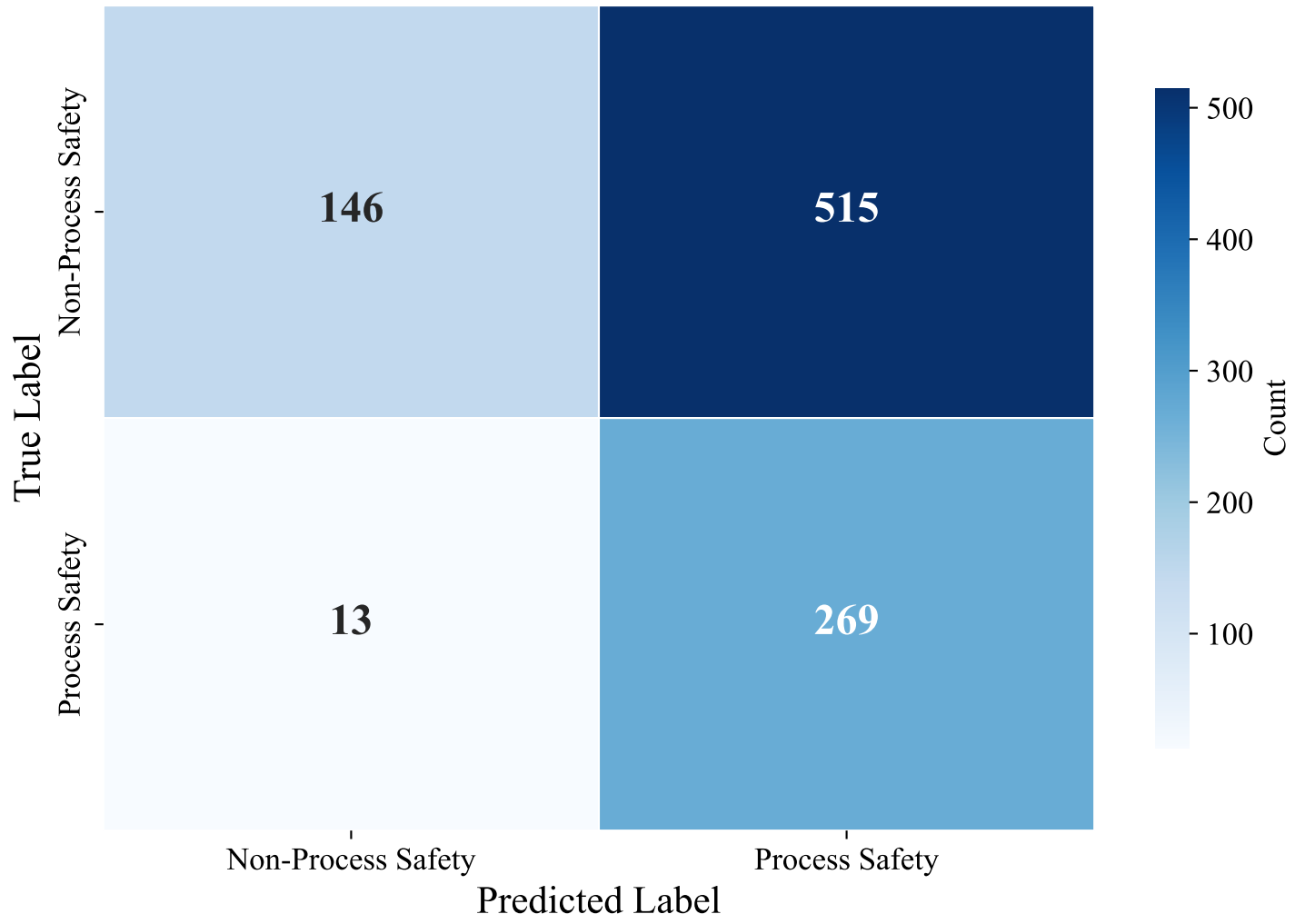
Confusion Matrix — ENGLISH_MANUAL (paraphrase-multilingual-MiniLM-L12-v2, random_forest)
