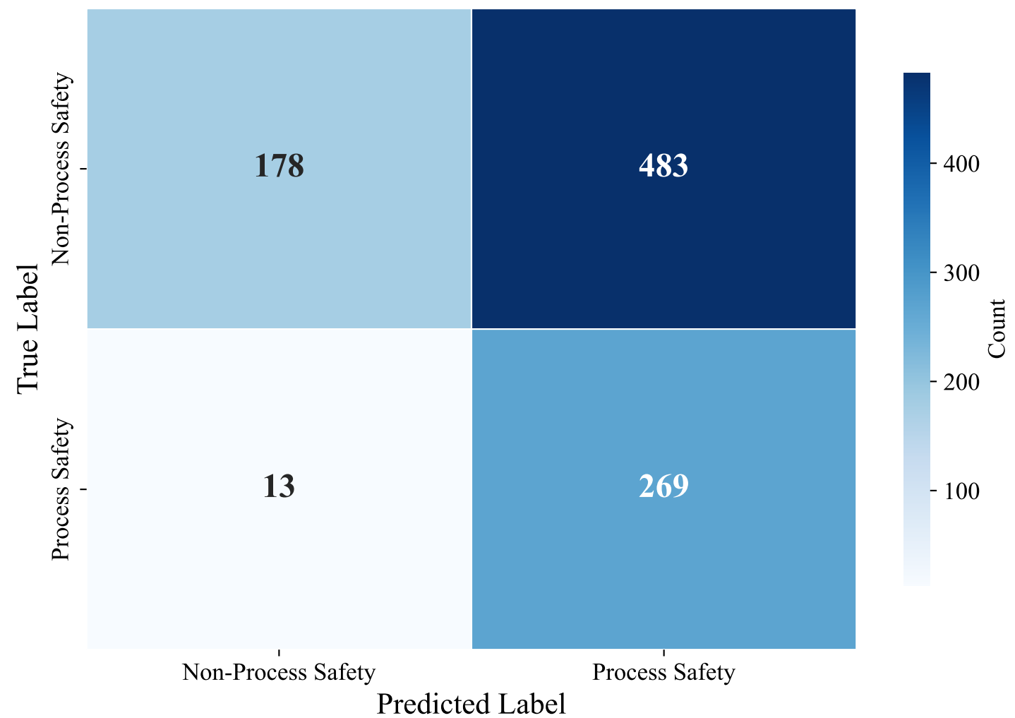
Confusion Matrix — ENGLISH_MANUAL (paraphrase-multilingual-MiniLM-L12-v2, svm_linear)
