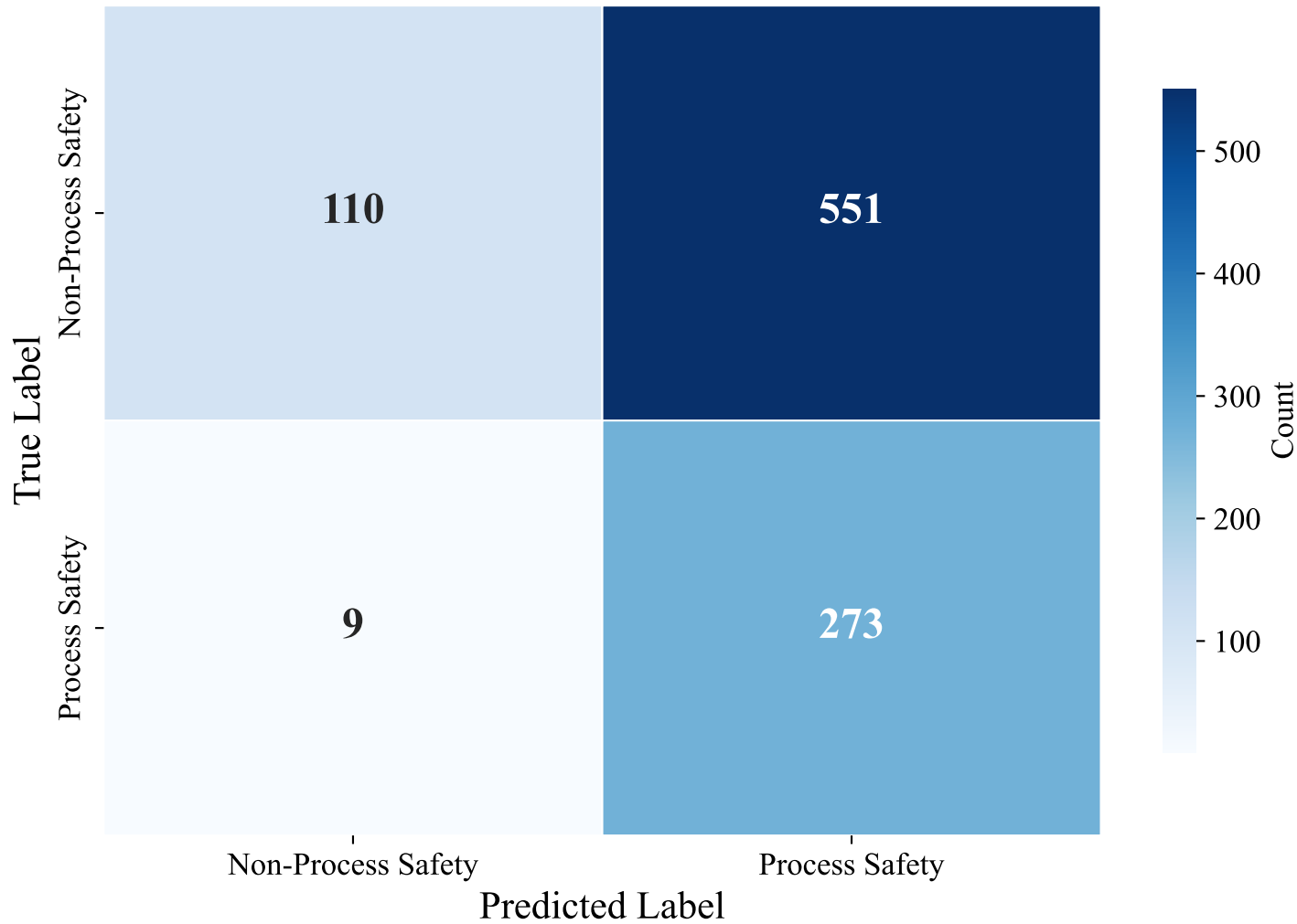
Confusion Matrix — ENGLISH_MANUAL (snowflake-arctic-embed-l-v2.0, random_forest)
