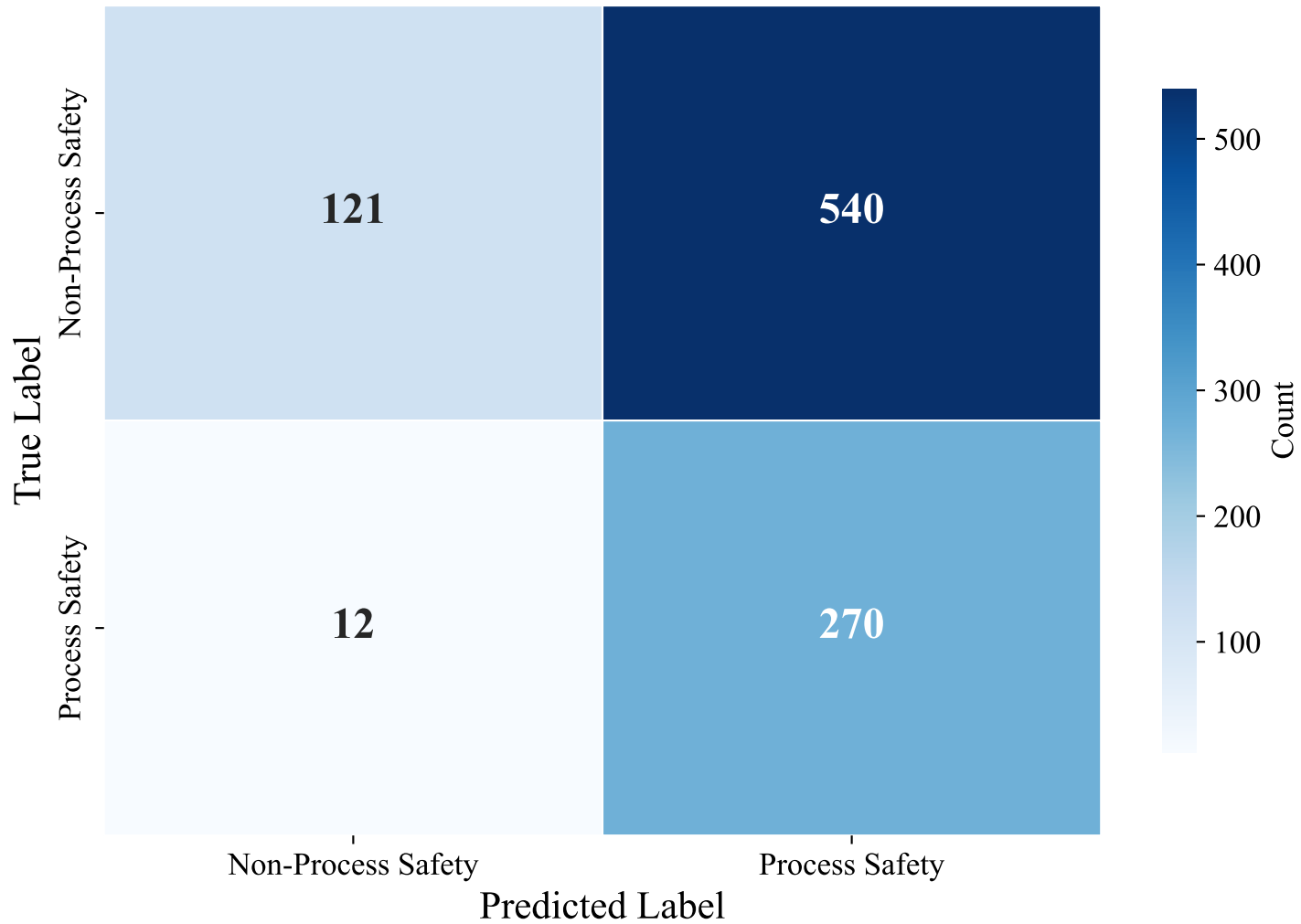
Confusion Matrix — ENGLISH_MANUAL (snowflake-arctic-embed-l-v2.0, xgboost)
