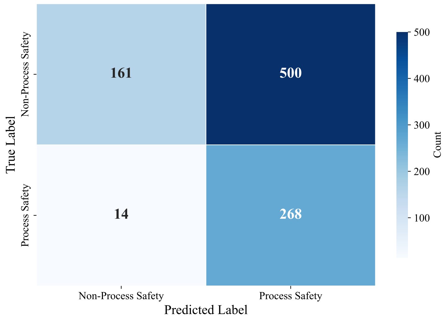
Confusion Matrix — ENGLISH_MANUAL (xlm-roberta-base, lightgbm)
