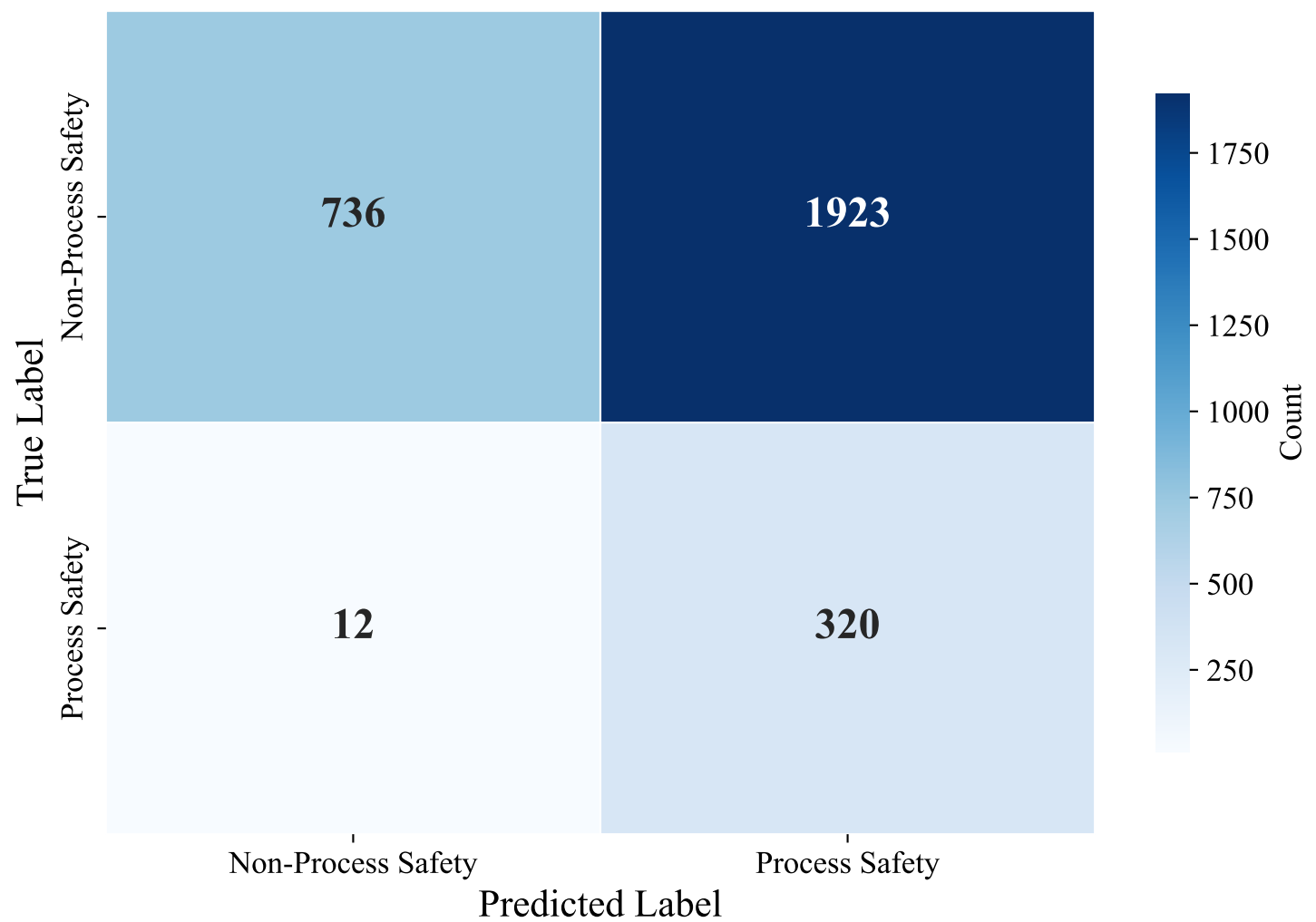
Confusion Matrix — GERMAN_MANUAL (multilingual-e5-large-instruct, svm_linear)
