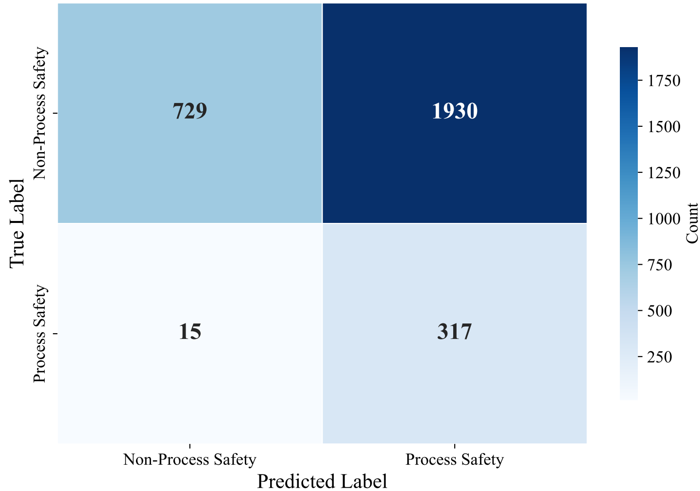
Confusion Matrix — GERMAN_MANUAL (multilingual-e5-large-instruct, xgboost)
