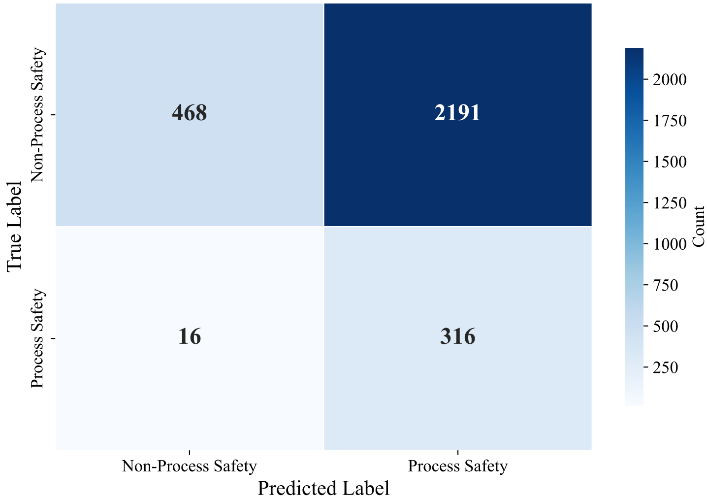
Confusion Matrix — GERMAN_MANUAL (paraphrase-multilingual-MiniLM-L12-v2, lightgbm)
