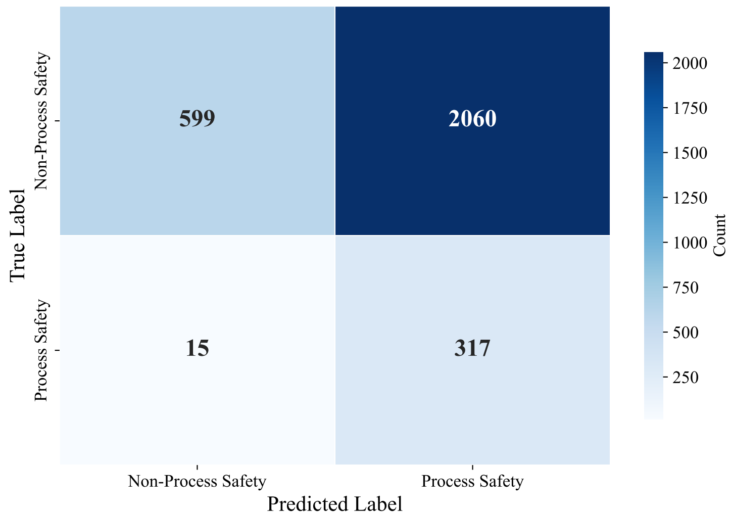
Confusion Matrix — GERMAN_MANUAL (paraphrase-multilingual-mpnet-base-v2, lightgbm)
