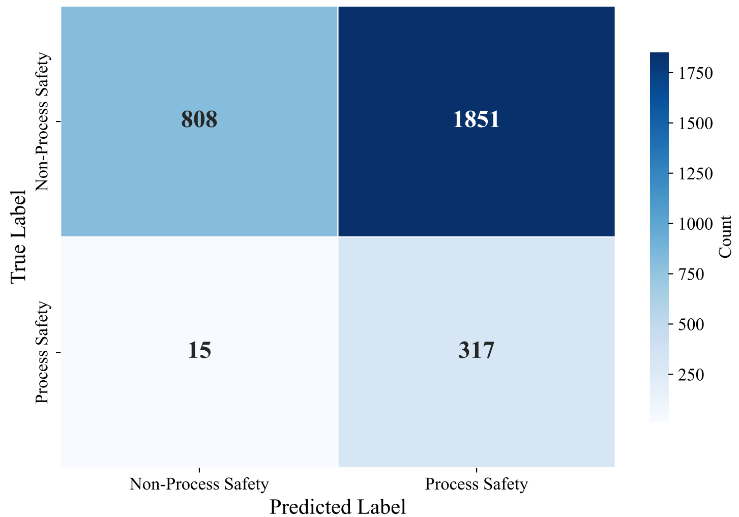
Confusion Matrix — GERMAN_MANUAL (snowflake-arctic-embed-l-v2.0, svm_rbf)
