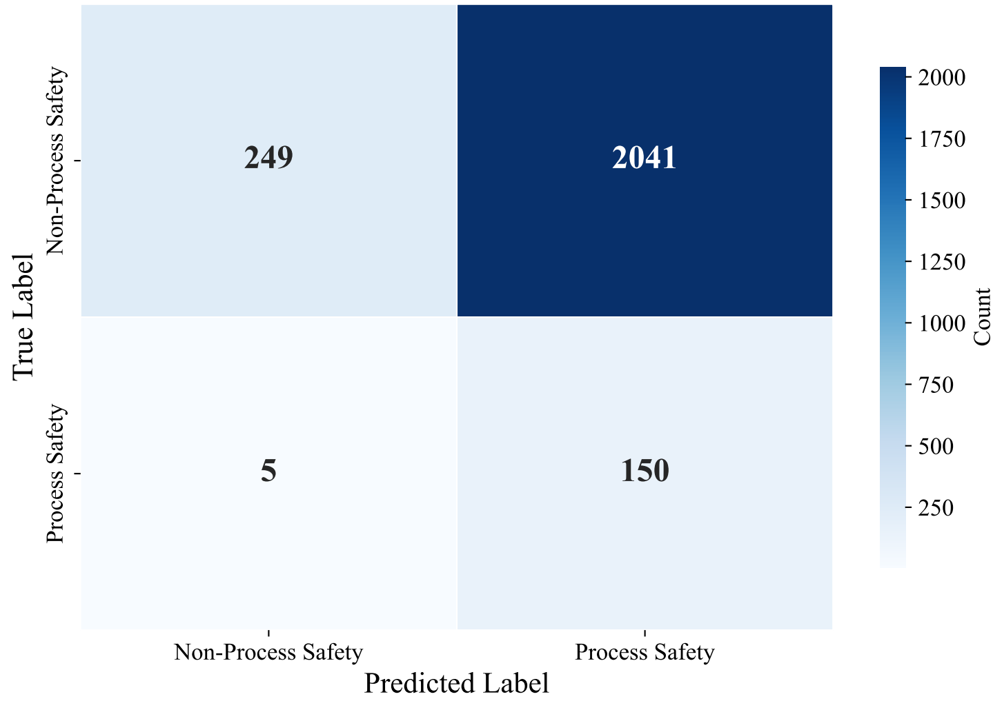
Confusion Matrix — SWEDISH_MANUAL (multilingual-e5-large-instruct, random_forest)
