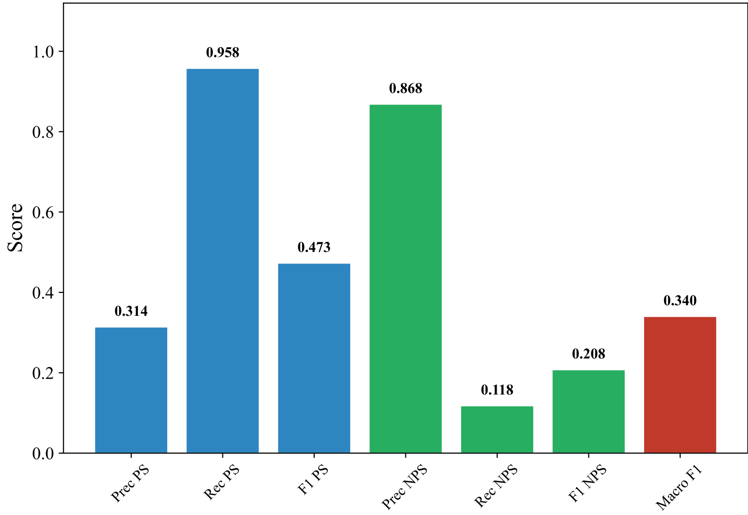
Classification Metrics — DUTCH_MANUAL (bert-base-multilingual-uncased, svm_linear)
