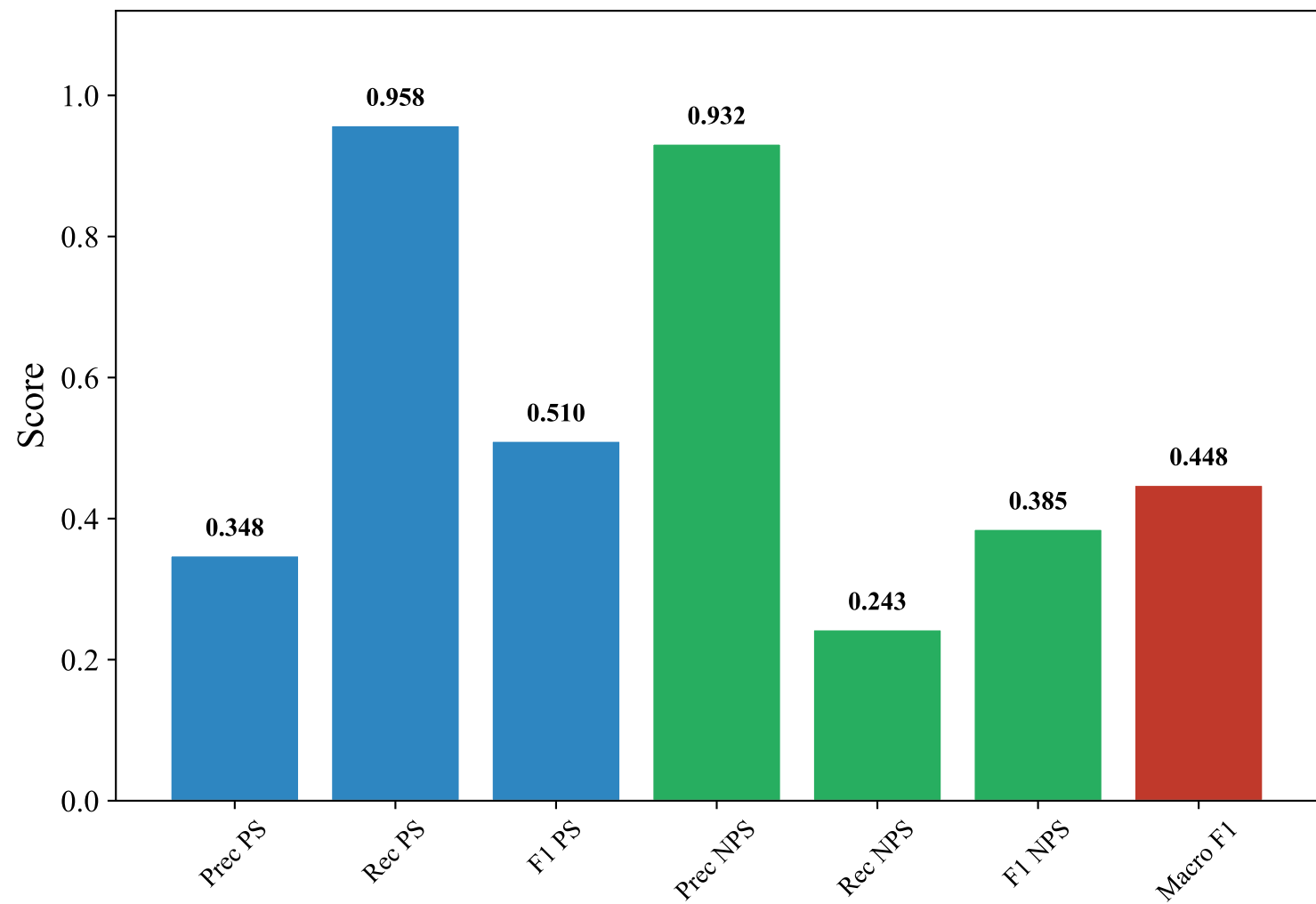
Classification Metrics — DUTCH_MANUAL (multilingual-e5-large-instruct, svm_linear)
